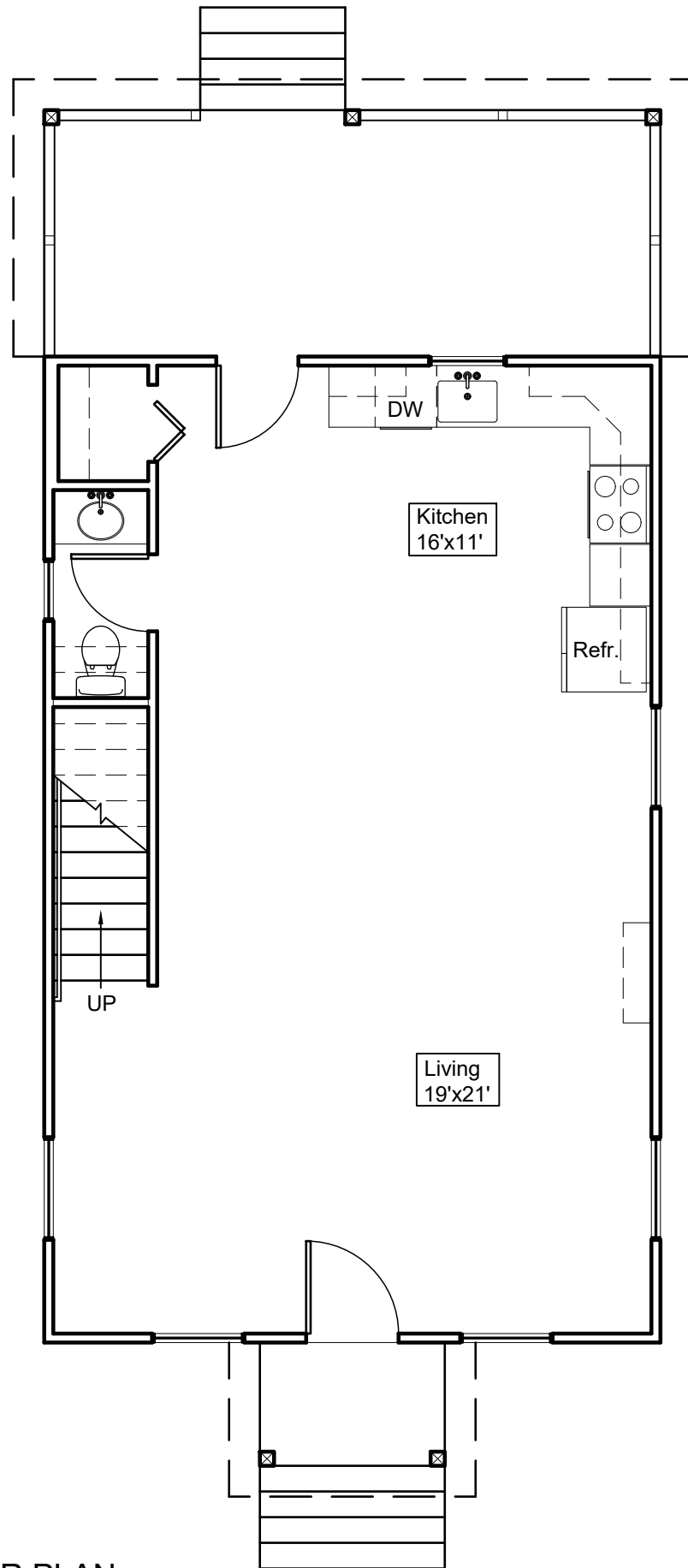
FIRST FLOOR PLAN 20'x32'
