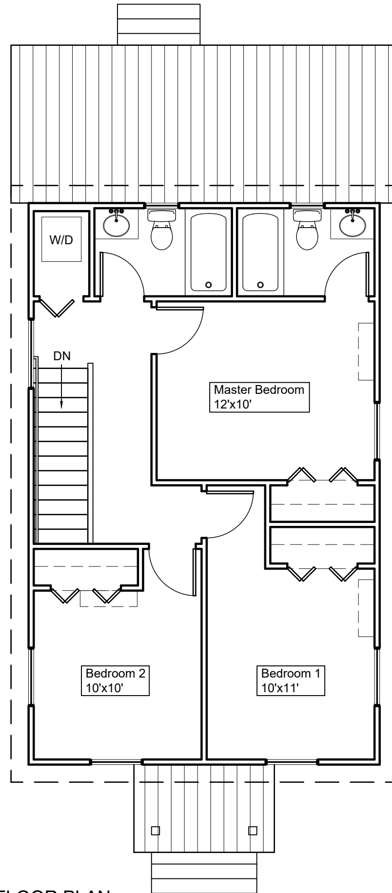
SECOND FLOOR PLAN 20'x32'
